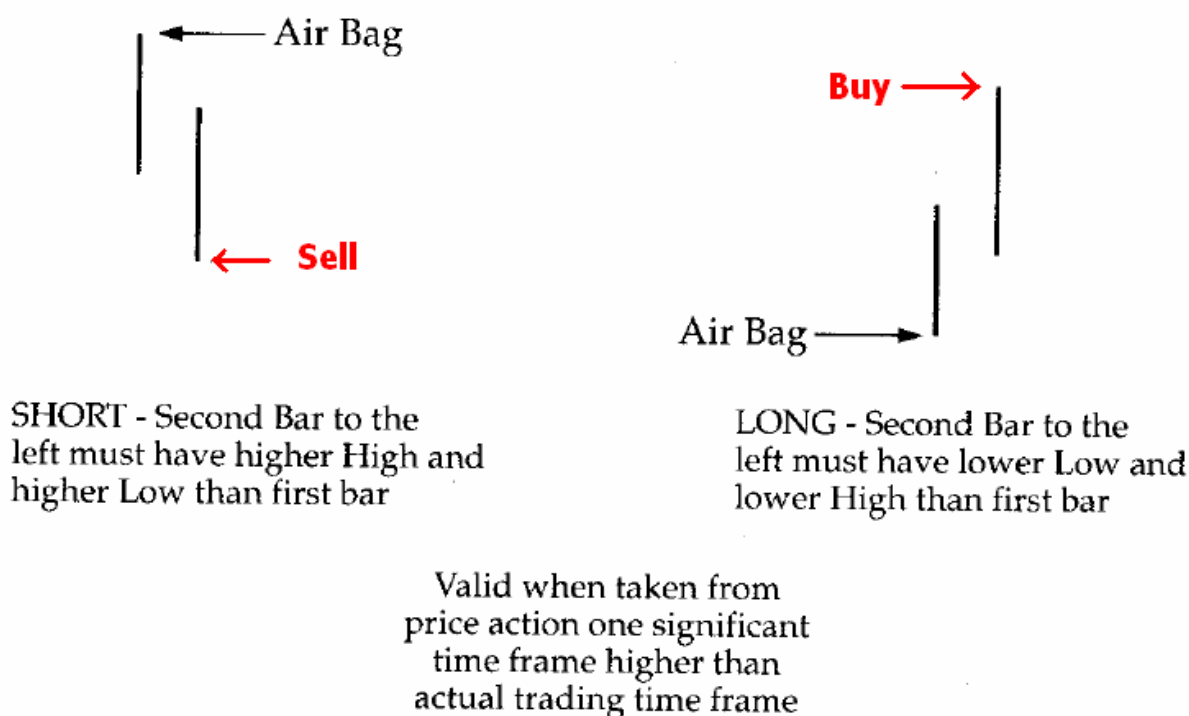
Figure 10-2 Two-bar reversals.
