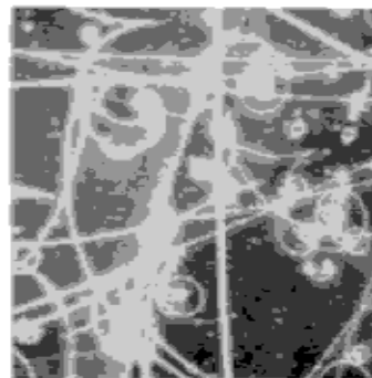
Atomic Particles in Bubble Chamber
